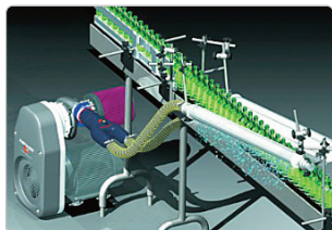
Air knives and low pressure blowers
